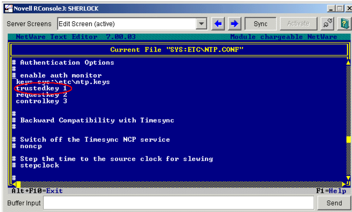
Figure 14 Ntp.conf File of ServerA
