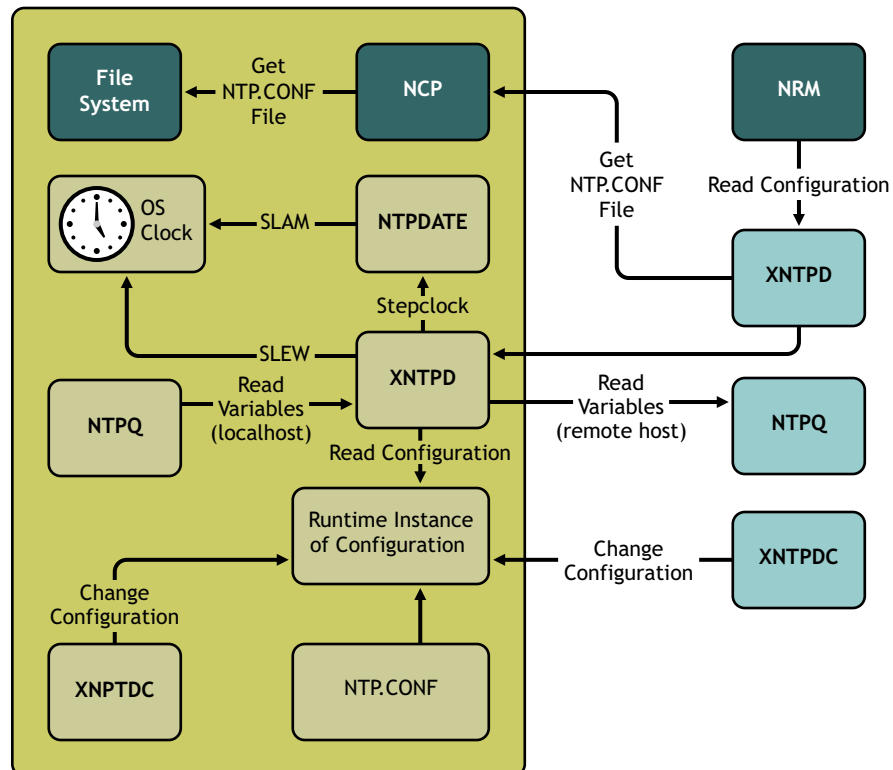
Figure 1 NTP Architecture
