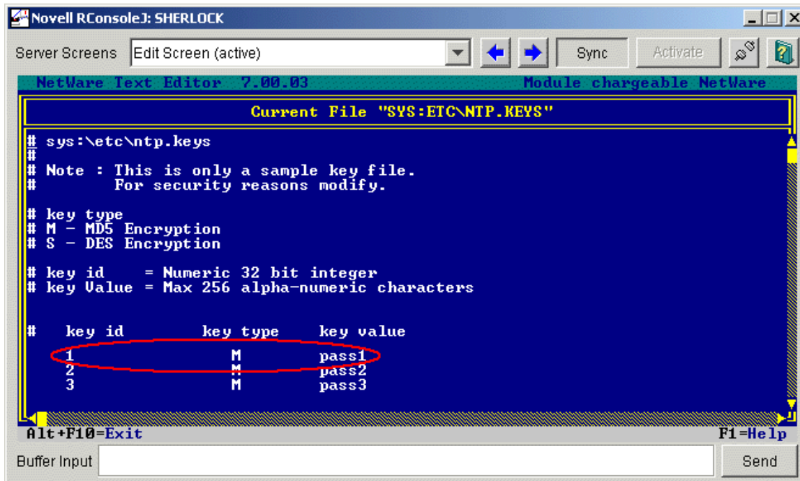
Figure 15 Ntp.keys File of ServerA
